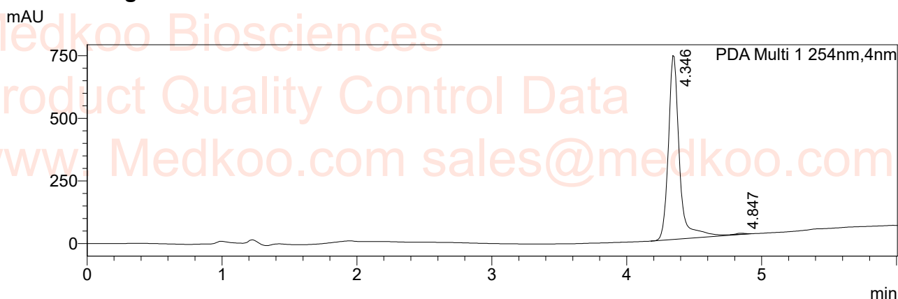
Peak Table
